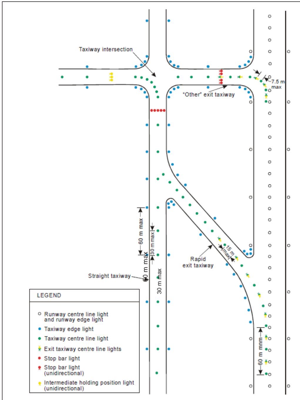
Figure 5-26. Taxiway lighting
