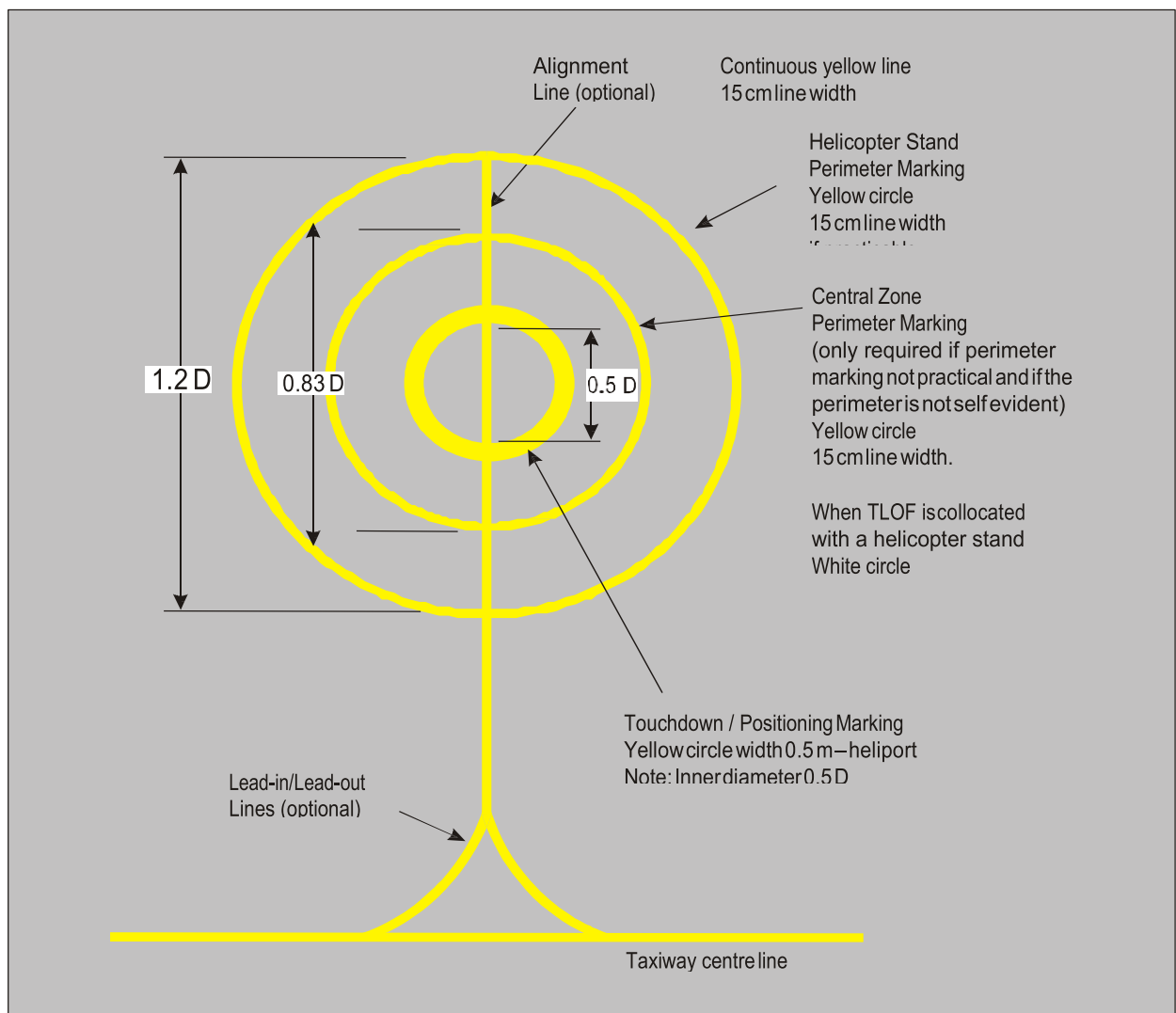
Figure 5-8. Helicopter stand markings
